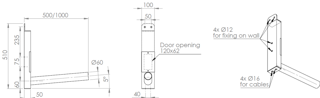
WALL BRACKET
