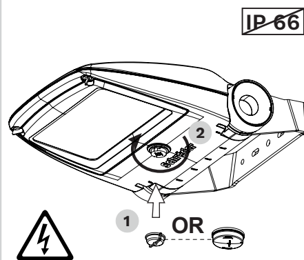
Zhaga bottom node or IP66 sealing cap
